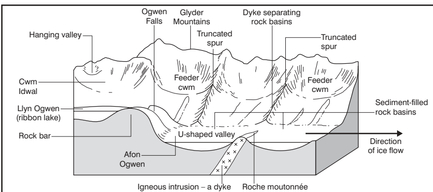
Figure 8: Block diagram of the Nant Ffroncon valley
