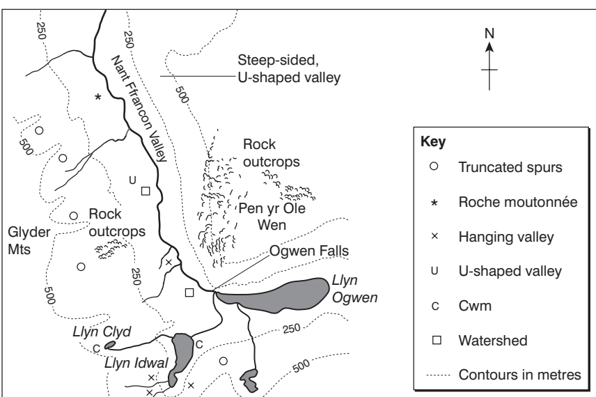
Figure 9: Sketch of the Nant Ffroncon Valley
